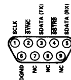
Figure 22. Pin Configuration for J2 (Front View)
