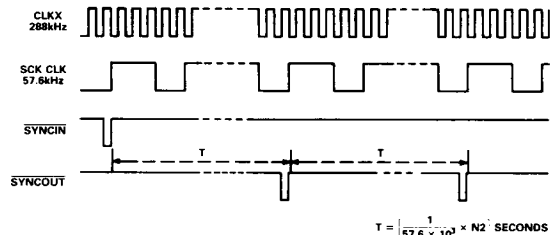
Figure 18. AD7341/AD7371 Timing Waveforms
