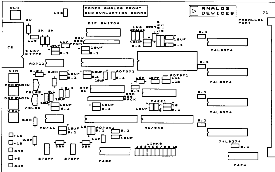
Figure 21. Component Overlay for Circuit of Figure 23
