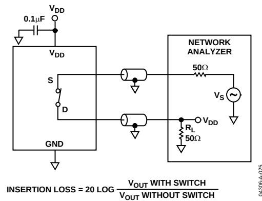
Figure 26. Bandwidth
