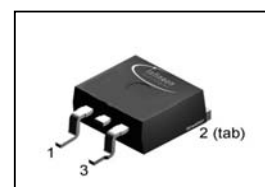
P-TO263-3
