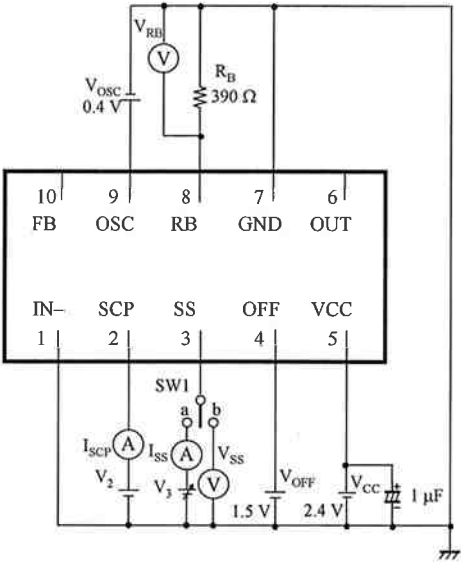
5. Test Circuit 5
