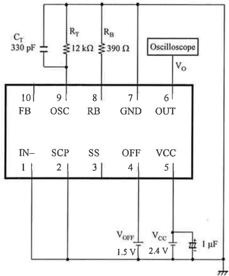
3. Test Circuit 3
