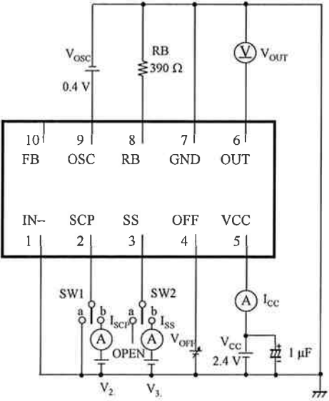
7. Test Circuit 7
