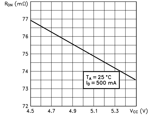
Figure 5: ON resistance vs. supply voltage (B)
