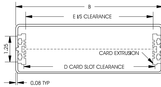
Front View - Panel Removed
