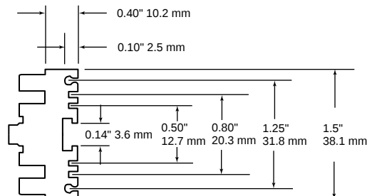
Right & Left Side Extrusion Detail
