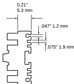
Right & Left Side Extrusion Detail
