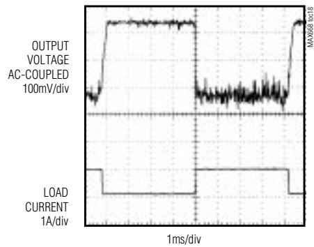
LOAD-TRANSIENT RESPONSE
