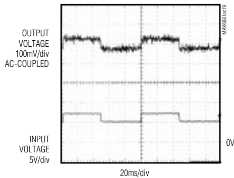
LINE-TRANSIENT RESPONSE
