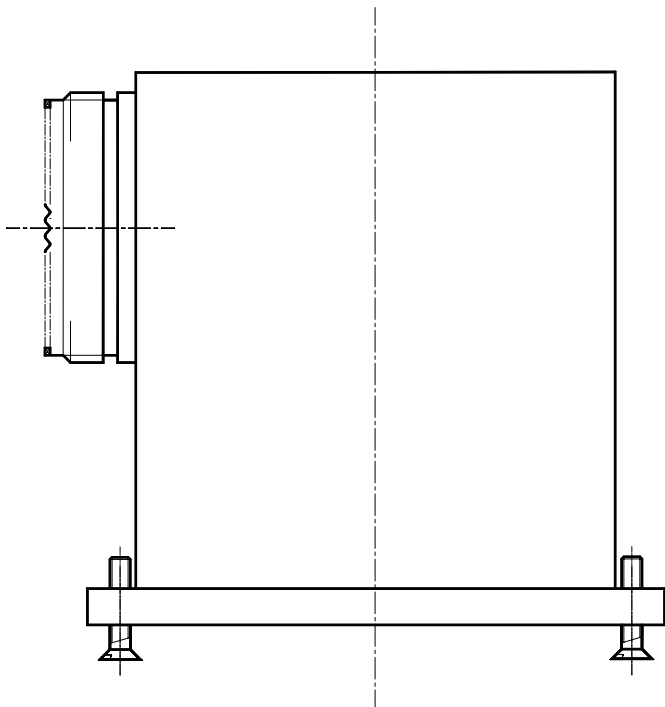
ADAPTER FOR MIL-C-81659 CONNECTOR
