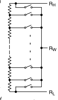
Figure 3. Electronic Potentiometer Implementation
