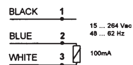
S5-1-x
