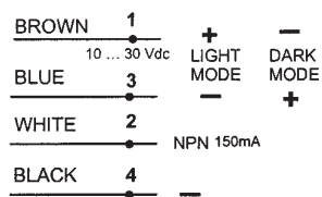
S5-5-x (4 wires)
