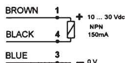
S5-5-x (3 wires)
