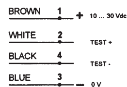
S5-5-G8/G12 (4 wires)
