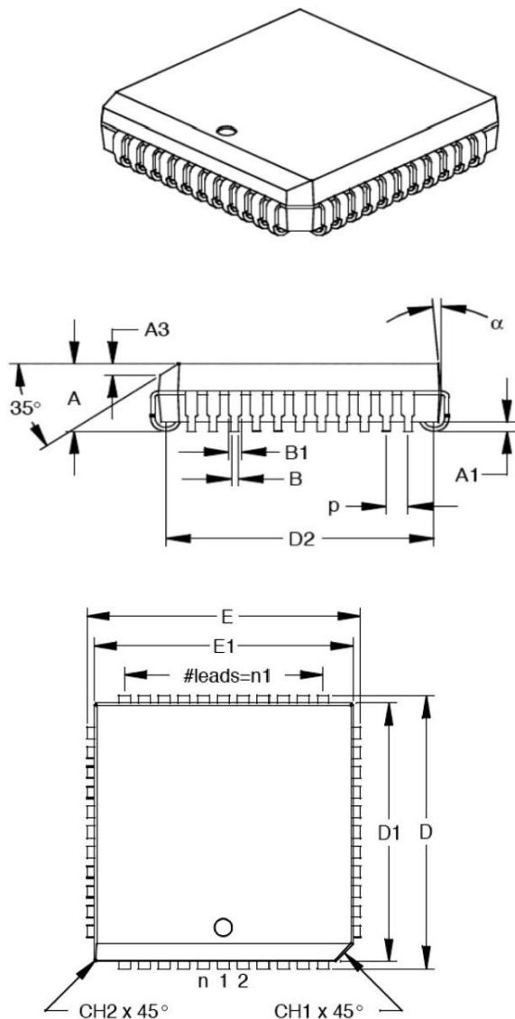
Figure 2. PLCC Physical Dimensions
