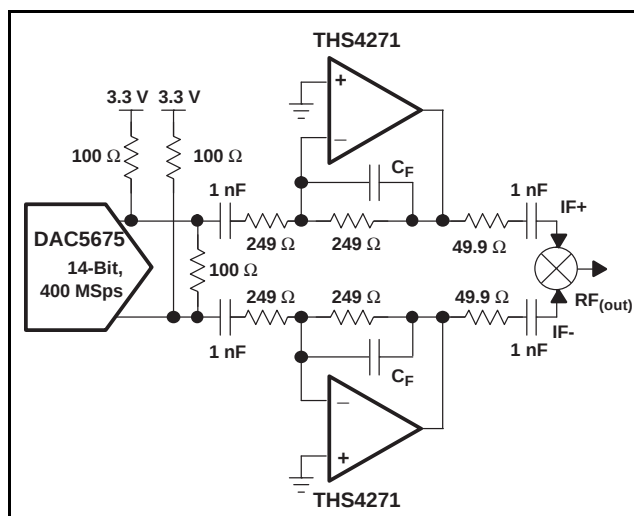
Figure 81. Differential Mixer Drive Circuit Using the DAC5675 and the THS4271
