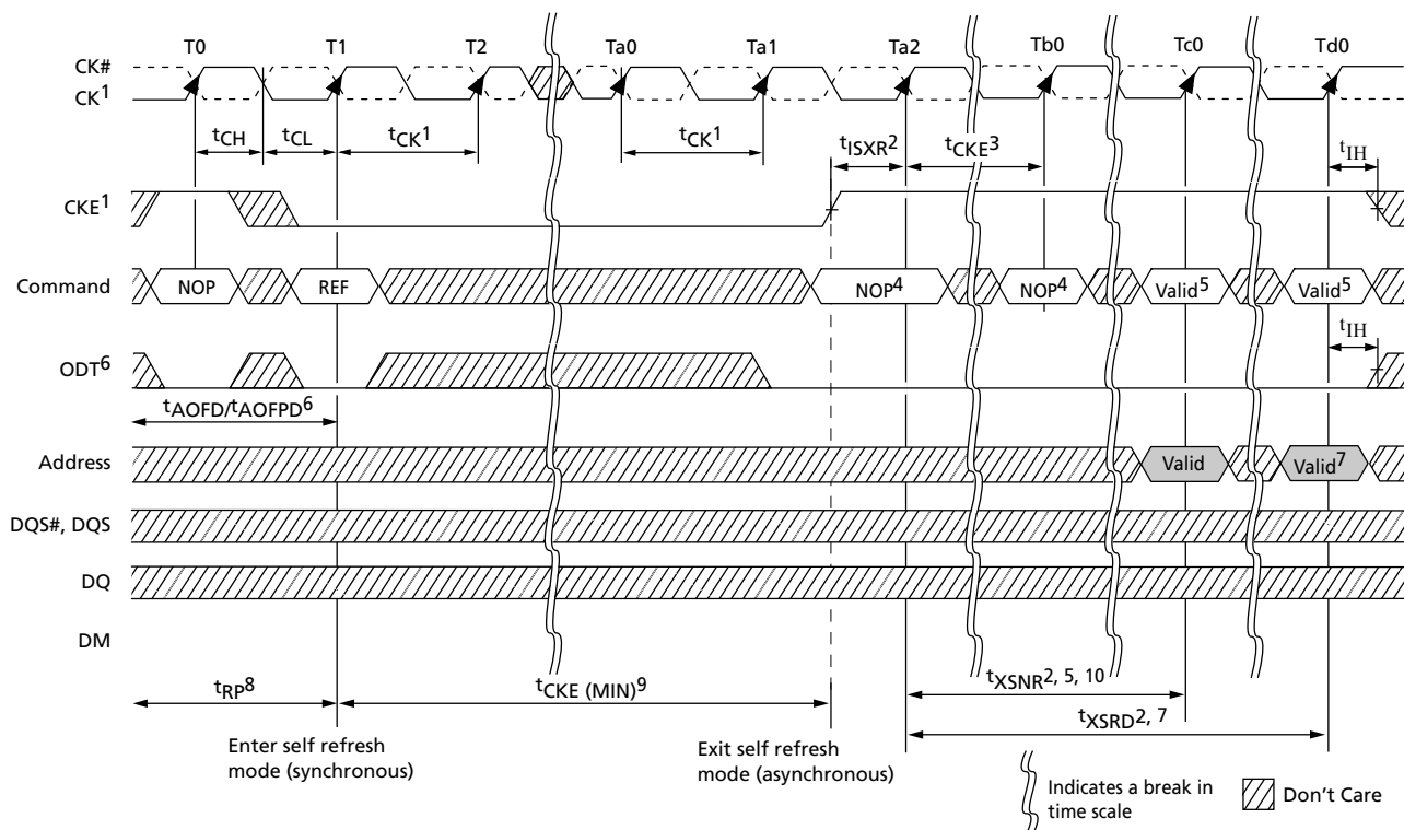
Figure 69: Self Refresh
