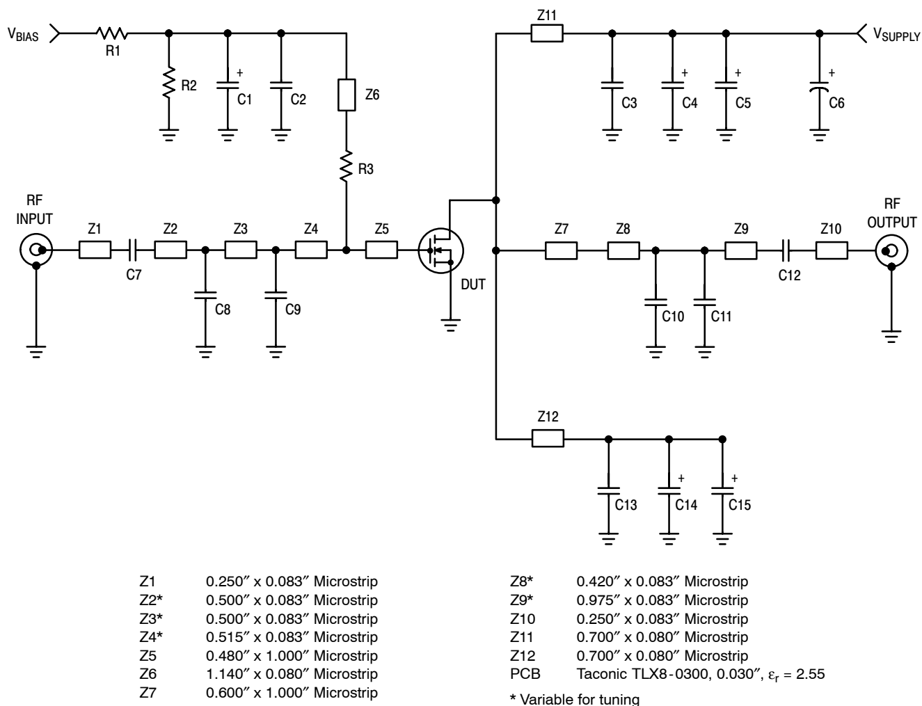
Figure 1. MRF5S19060NR1/NBR1 Test Circuit Schematic
