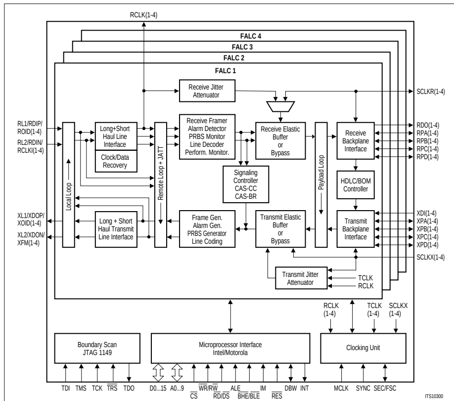
Figure 5 Block Diagram
