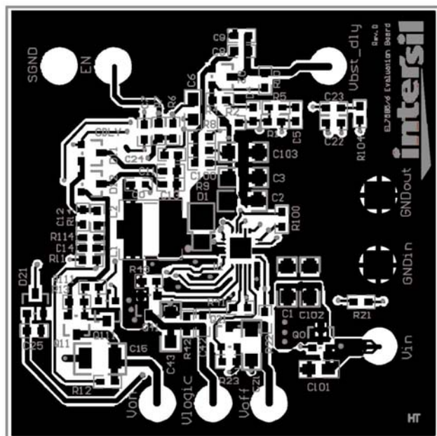
FIGURE 35. TOP LAYER
