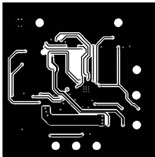
FIGURE 36. BOTTOM LAYER
