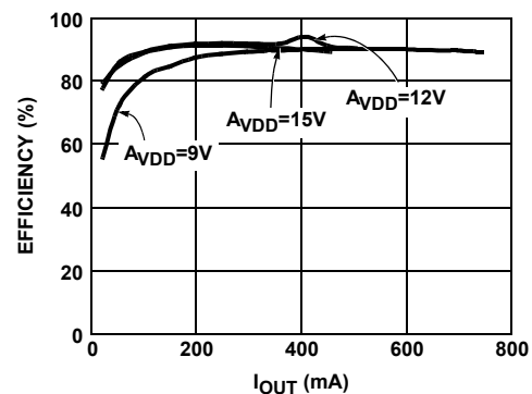
FIGURE 4. VBOOST EFFICIENCY AT V_{IN} = 5V (P MODE)
