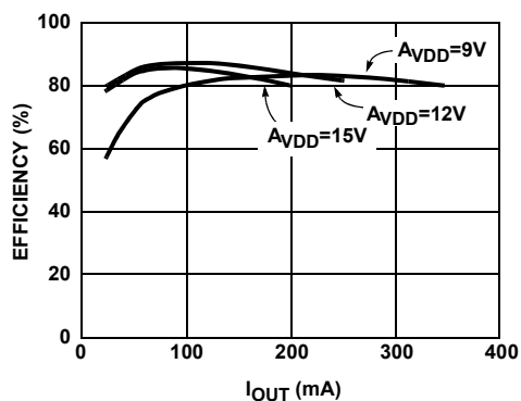
FIGURE 1. VBOOST EFFICIENCY AT V_{IN} = 3V (PI MODE)
