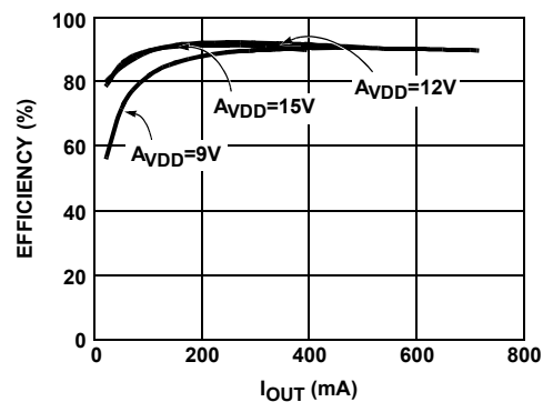
FIGURE 2. VBOOST EFFICIENCY AT V_{IN} = 5V (PI MODE)
