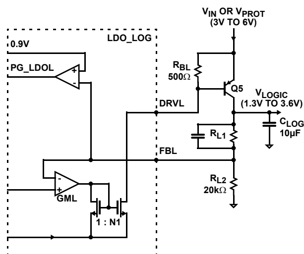
FIGURE 30. V_{\text{LOGIC}} FUNCTIONAL BLOCK DIAGRAM
