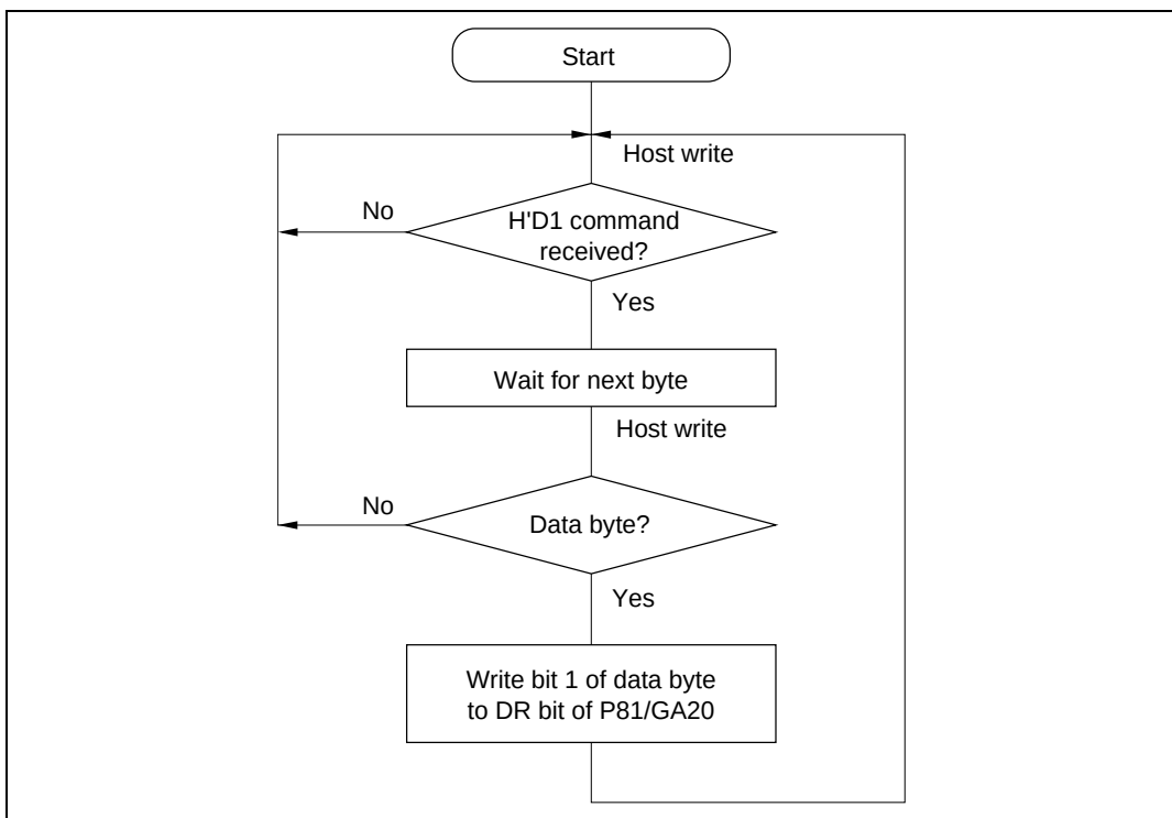
Figure 18.2 GA20 Output
