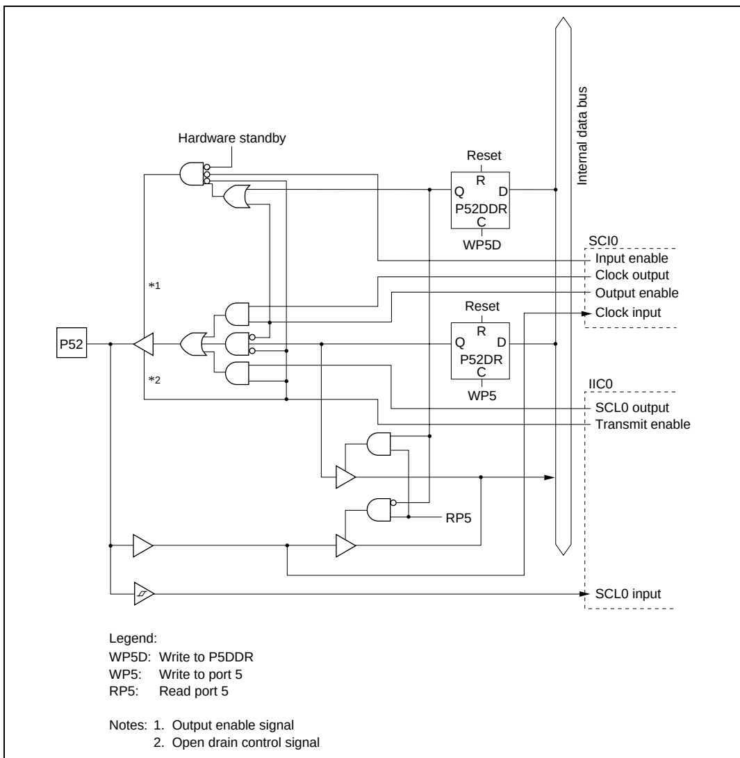
Figure C.15 Port 5 Block Diagram (Pin P52)
