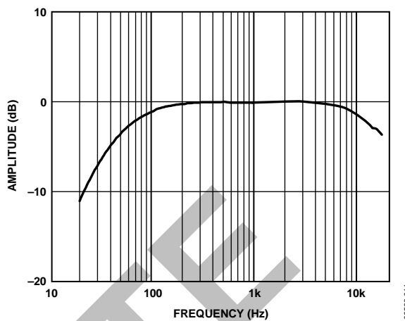
Figure 8. Typical Frequency Response (Measured)
