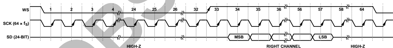
Figure 12. Mono Output I²S Format Right Channel (L/R = 1)
