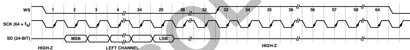
Figure 11. Mono Output I²S Format Left Channel (L/R = 0)
