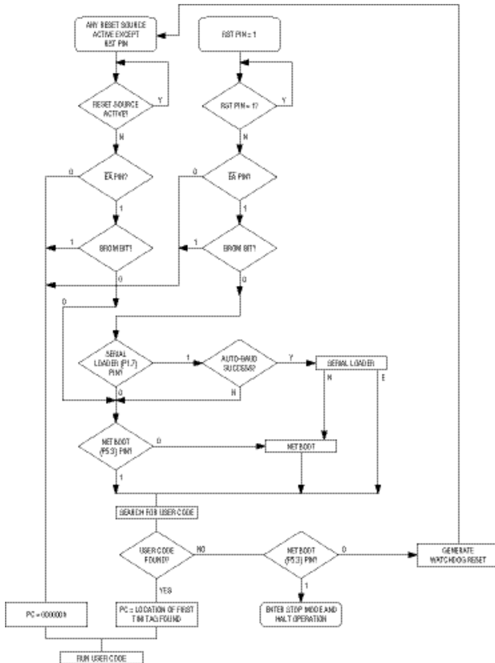
Figure 12. ROM Code Boot Sequence
