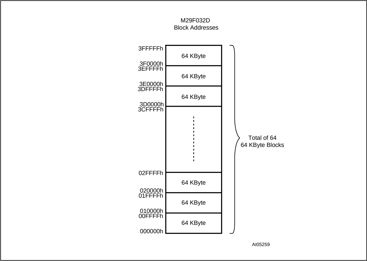
Figure 4. Block Addresses
