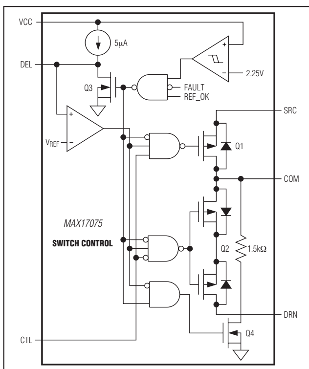
Figure 7. Switch Control
