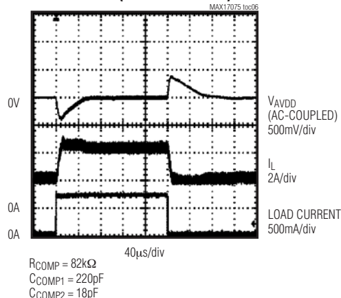
STEP-UP REGULATOR LOAD-TRANSIENT RESPONSE (100mA TO 800mA)
