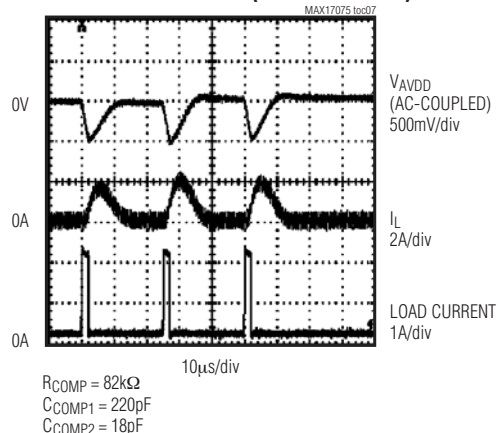
STEP-UP REGULATOR PULSED LOAD-TRANSIENT RESPONSE (80mA TO 2.08mA)
