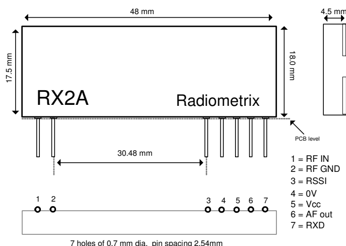
Figure 5: Physical dimensions
