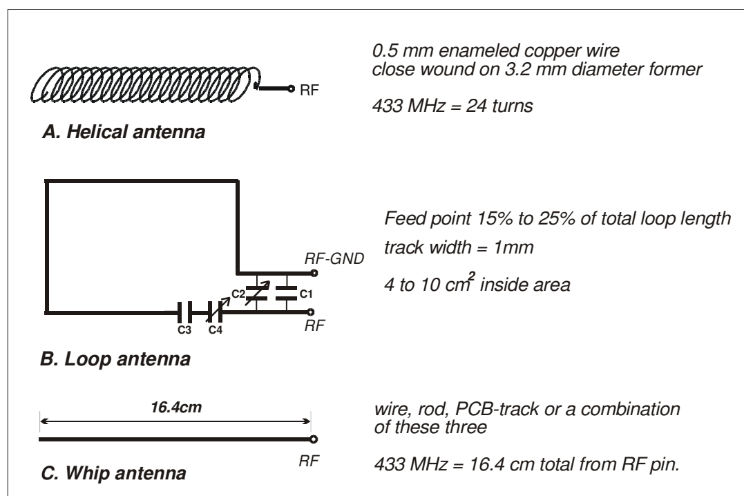
Fig.7: Antenna configuration
