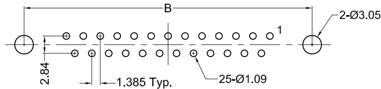
Recommended PCB Layout (Top View)
