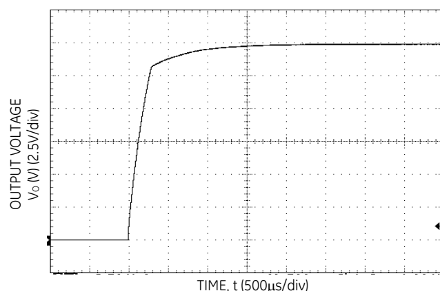
Figure 6. Typical Start-Up Output Voltage Rise Characteristic.
