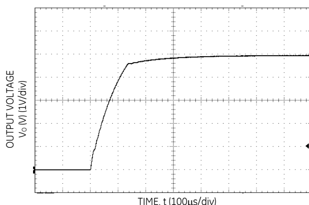
Figure 18. Typical Start-Up Output Voltage Rise Characteristic.
