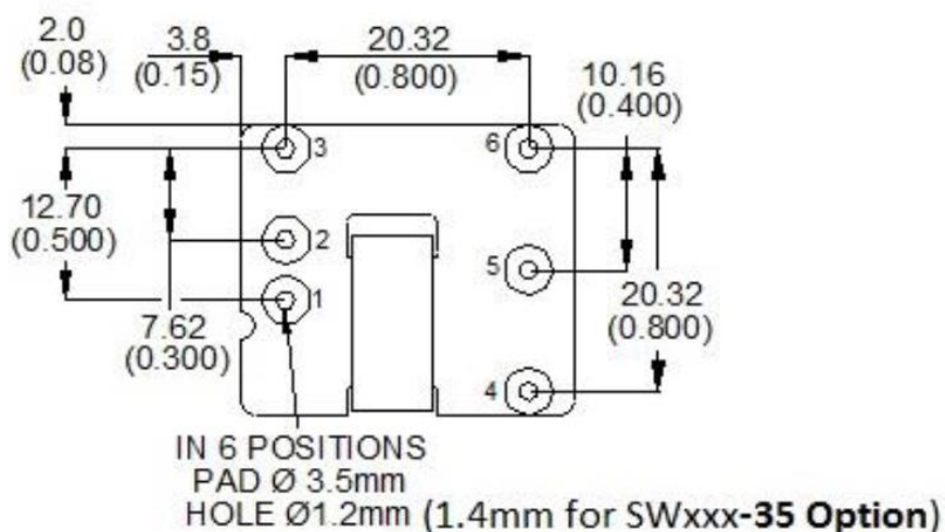
Through-Hole Pad Layout – Component side view
