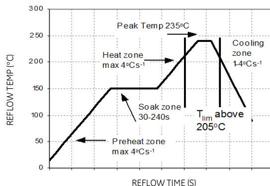
Figure 55. Time Limit, T_{lim} , Curve Above 205°C Reflow .
