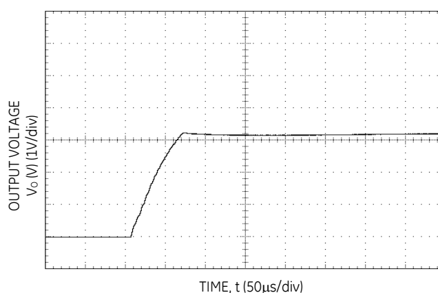
Figure 42. Typical Start-Up Output Voltage Rise Characteristic.
