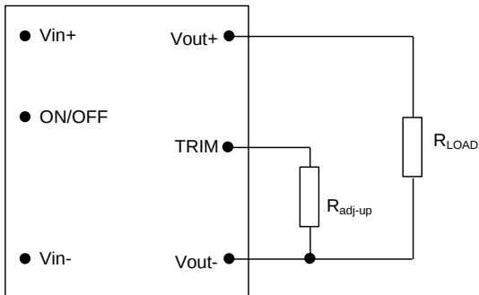
Figure 48. Circuit Configuration to Increase Output Voltage.
