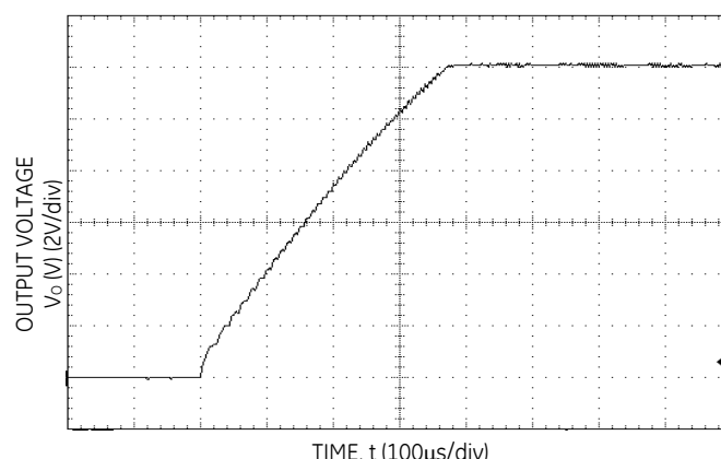
Figure 30. Typical Start-Up Output Voltage Rise Characteristic.
