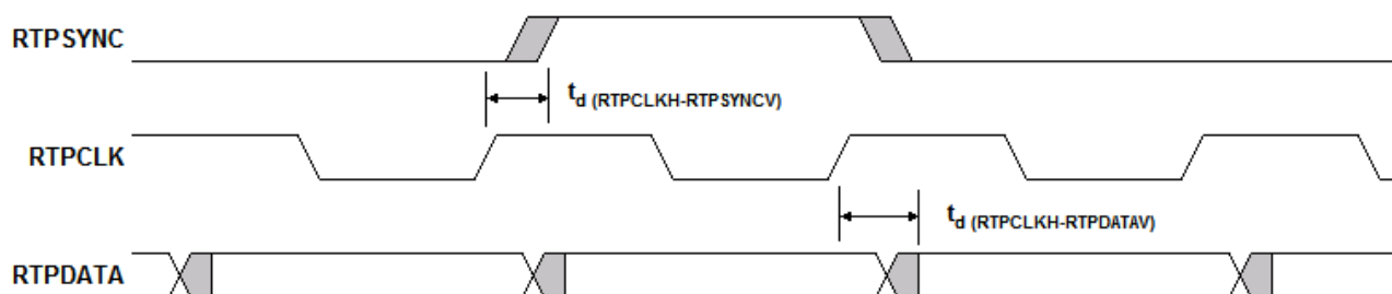
Figure 4-25. RTPDATA Timing
