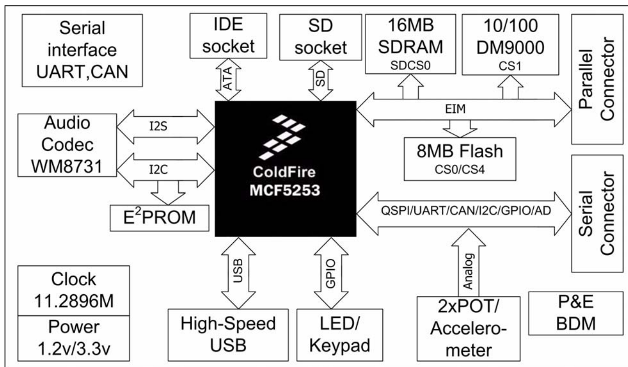
Figure 1. M5253 Demo Board Block Diagram
