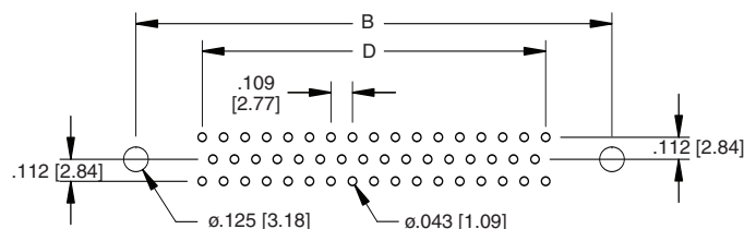
Recommended PCB Layout 50 Position
