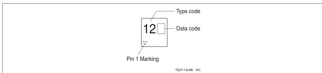
Figure 7 Marking Layout
