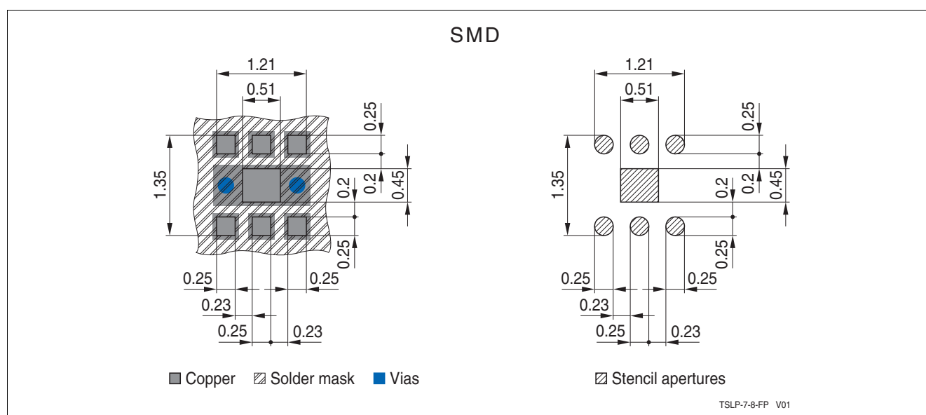
Figure 6 Footprint TSLP-7-8
