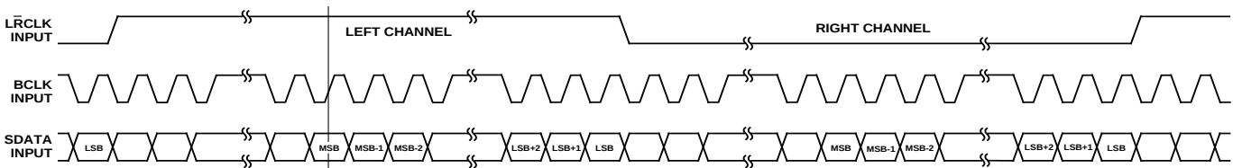
Figure 2. Right-Justified Mode
