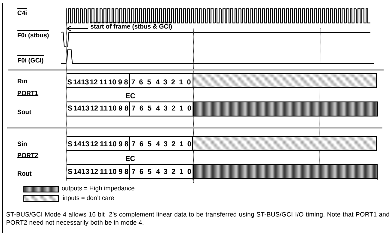
Figure 6 - ST-BUS and GCI 16-Bit 2's Complement Linear PCM I/O (Mode 4)
