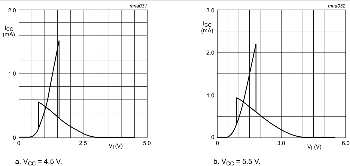
Fig. 7. Typical 74HCT3G14-Q100 transfer characteristics
