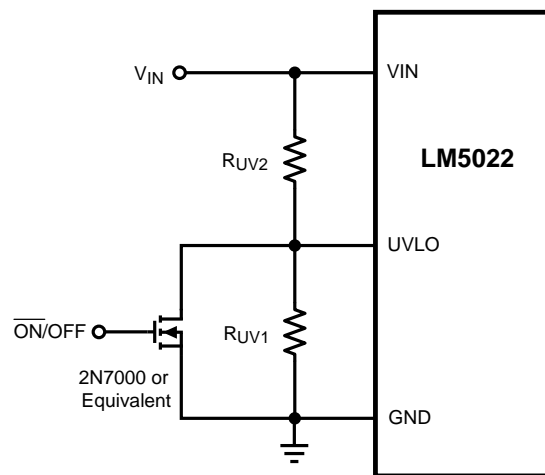
Figure 13. Enable/Disable Using UVLO
