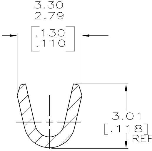
SECTION Y-Y SCALE 10:1
