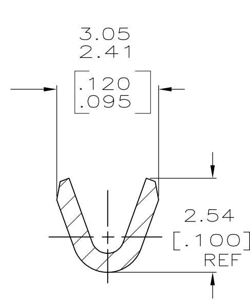
SECTION X-X SCALE 10:1
