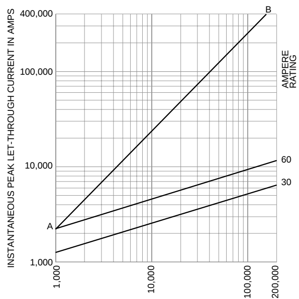
Current-Limitation Curves
