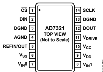
Figure 3. TSSOP Pin Configuration
