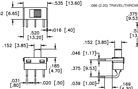
MECHANICAL OUTLINE
