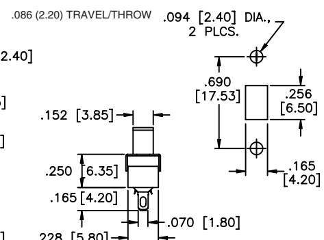
MECHANICAL OUTLINE
