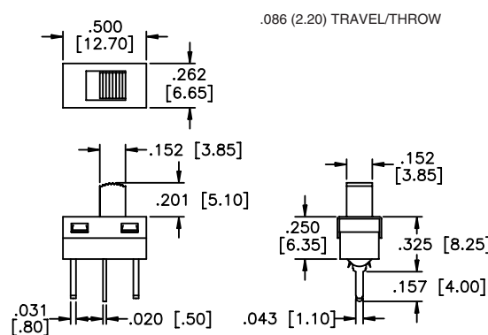
MECHANICAL OUTLINE
