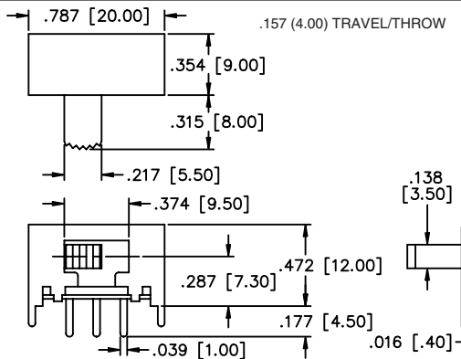
MECHANICAL OUTLINE
