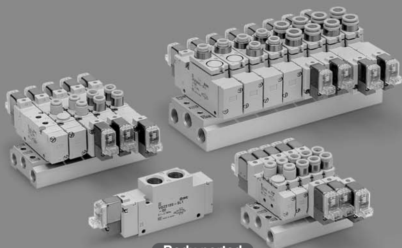
Body ported
