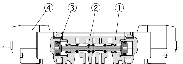
2 position double
