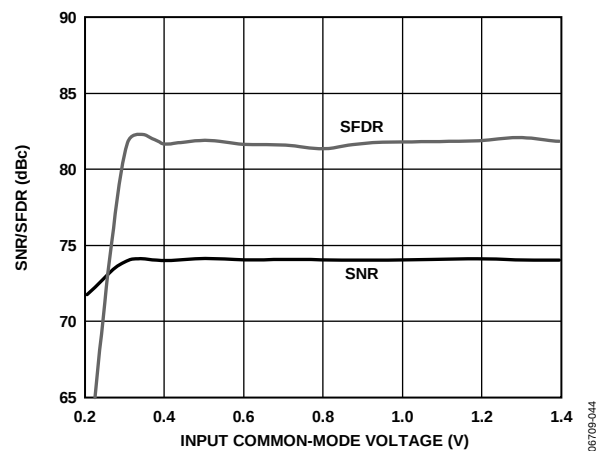
Figure 45. AD6655-150 SNR/SFDR vs. Input Common Mode ( V_{CM} ) with f_{IN} = 30.3\text{ MHz} , f_{NCO} = 45\text{ MHz}
