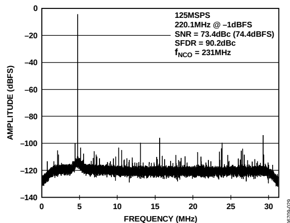
Figure 30. AD6655-125 Single-Tone FFT with f_{IN} = 220.1\text{ MHz} , f_{NCO} = 231\text{ MHz}
