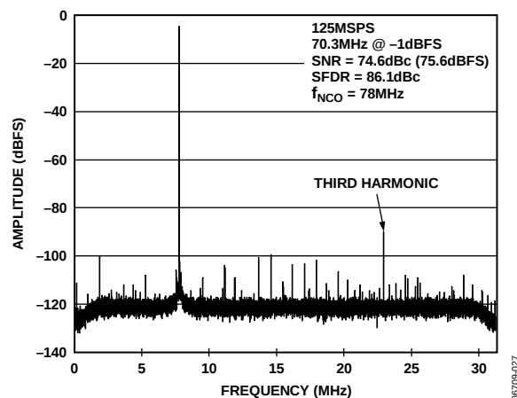
Figure 28. AD6655-125 Single-Tone FFT with f_{IN} = 70.3\text{ MHz} , f_{NCO} = 78\text{ MHz}
