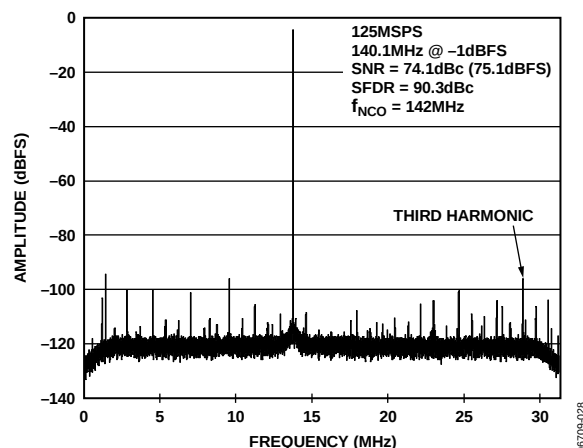
Figure 29. AD6655-125 Single-Tone FFT with f_{IN} = 140.1\text{ MHz} , f_{NCO} = 142\text{ MHz}
