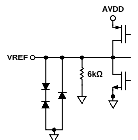
Figure 18. Equivalent VREF Circuit
