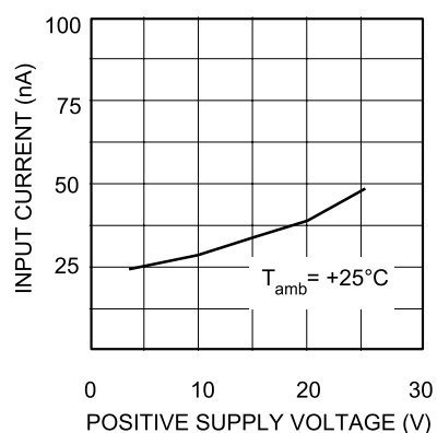
Figure 15. Input current
