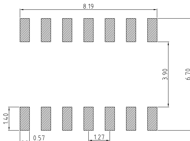
Figure 29. SO-14 recommended footprint
