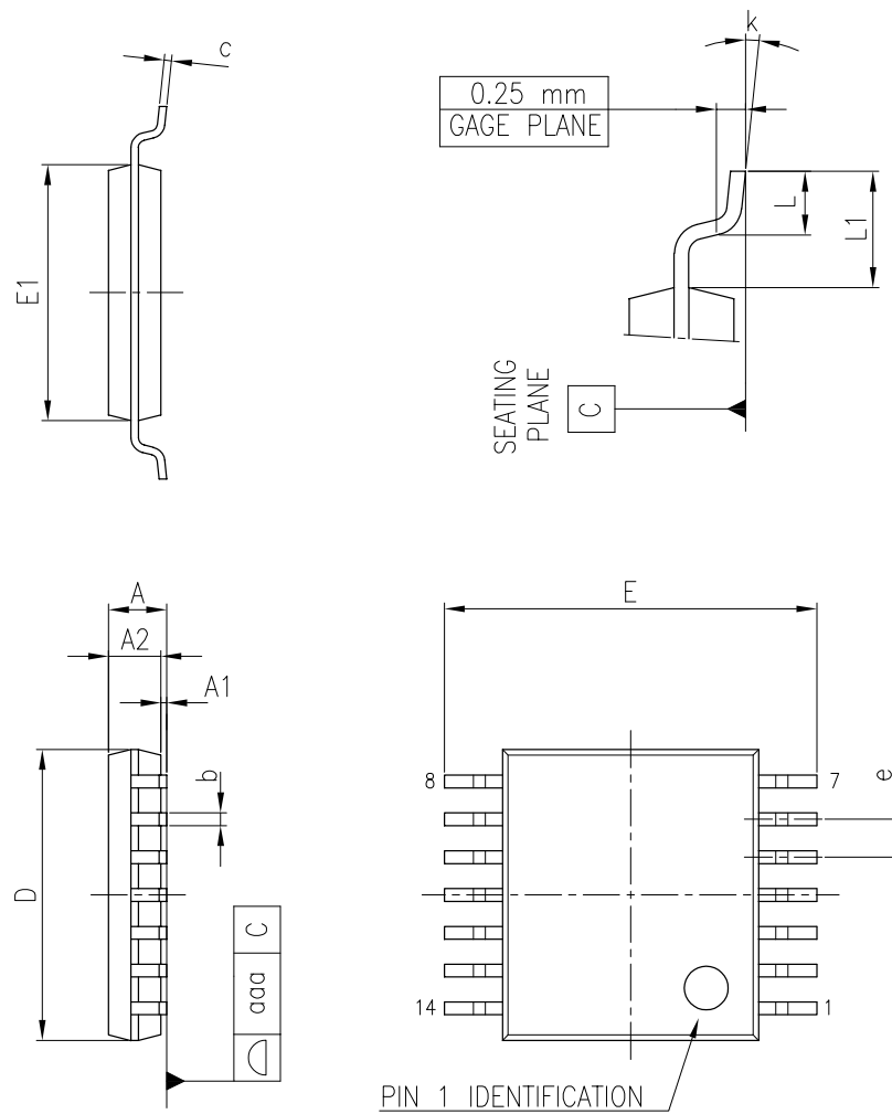
Figure 30. TSSOP-14 package outline
