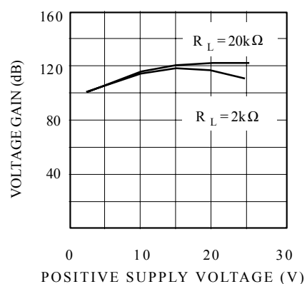
Figure 16. Voltage gain
