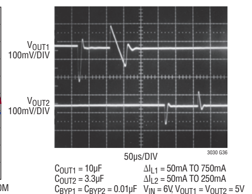
Channel-to-Channel Isolation
