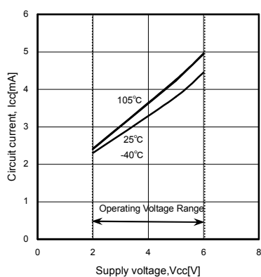
Fig.1 Circuit current
