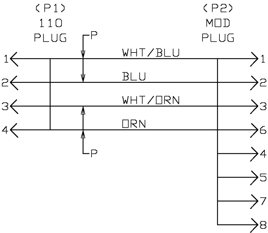
WIRING DIAGRAM 10 BASE-T
