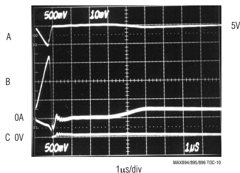
CURRENT-LIMIT RESPONSE (MAX894L, R_L = 0.7\Omega )
