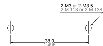
Panel cutout
