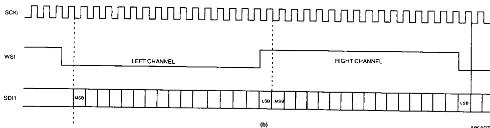
Fig.3 I²S 4 fs input formats.
