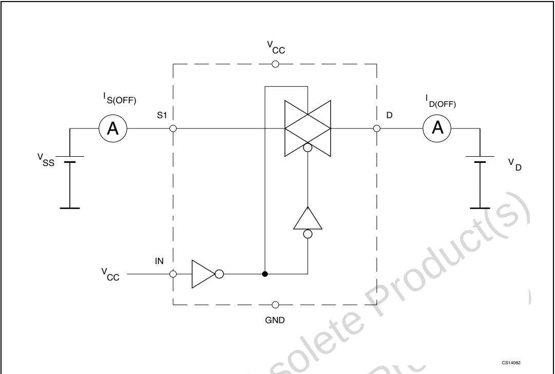
Figure 4. OFF leakage
