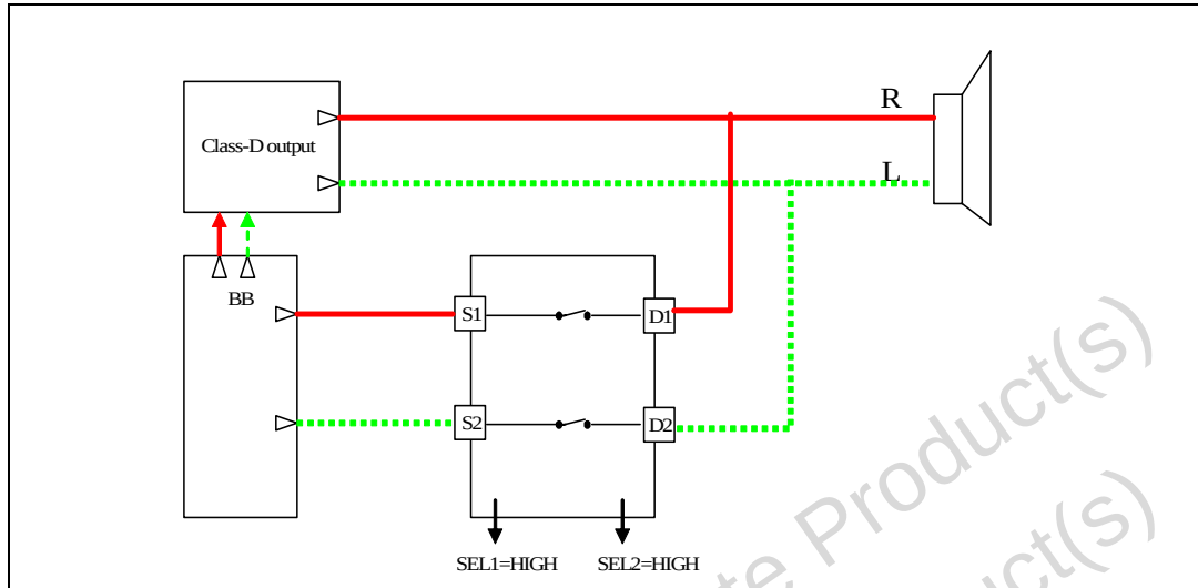
Figure 9. Application diagram
