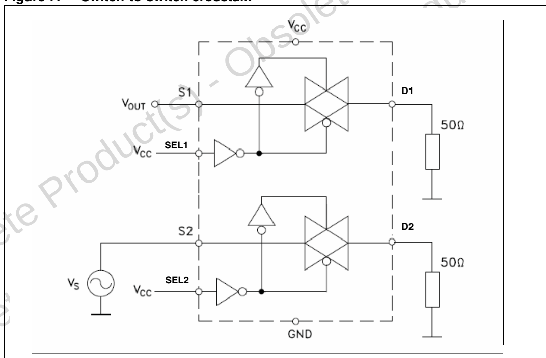
Figure 7. Switch-to-switch crosstalk
