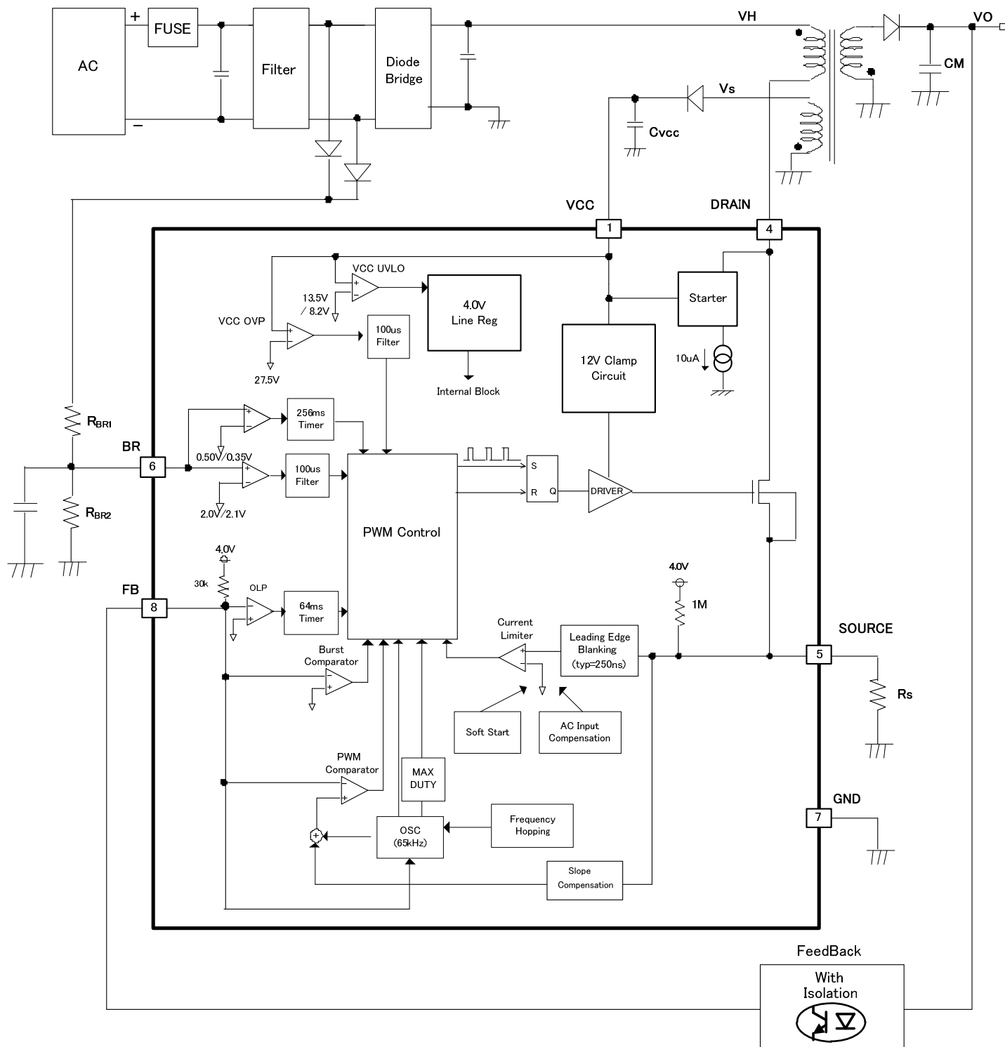
Figure 3. Block Diagram
