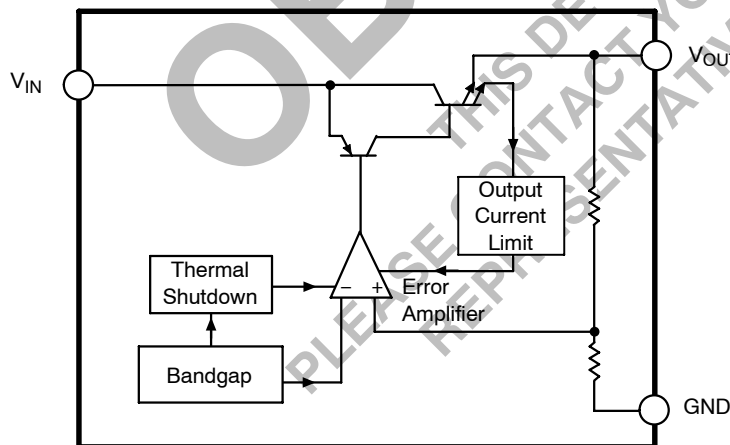
Figure 1. Block Diagram
