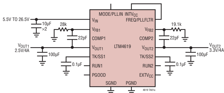
Dual 4A 3.3V/2.5V DC/DC \mu Module Regulator
