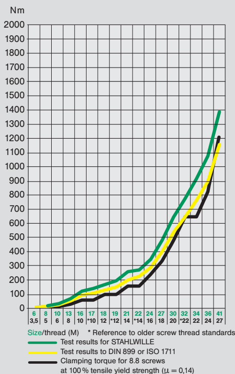
Guaranteed test results STAHLWILLE combination spanners No 13 (open-jaw)
