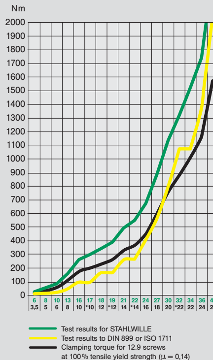
Guaranteed test results STAHLWILLE combination spanners No 13 (ring)
